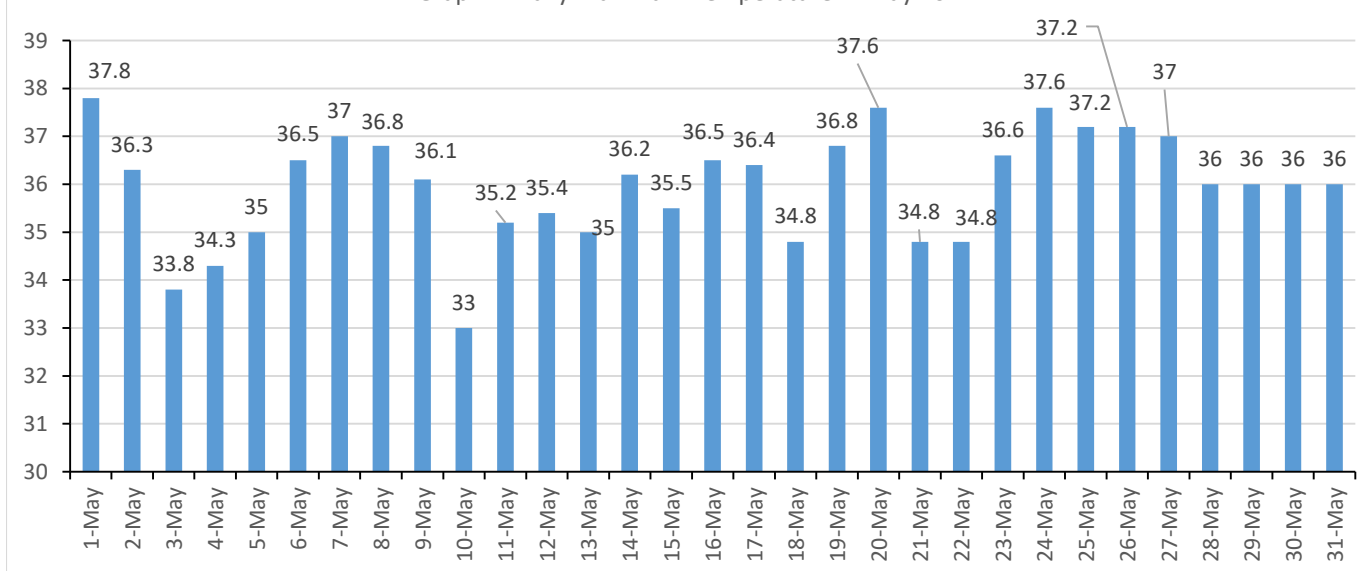
Graph 2: Daily Maximum Temperature in May 2022
